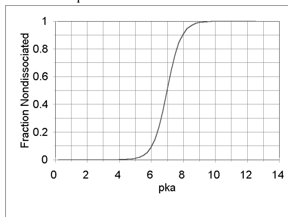
Figure 133. Dissociation as a function of pK_a at an ambient pH of 7
