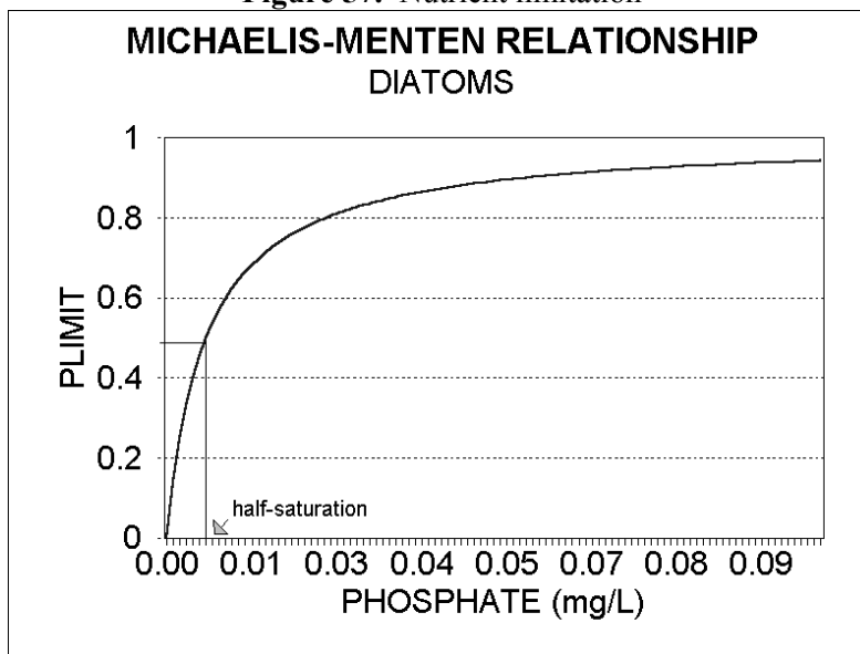
Figure 57. Nutrient limitation
