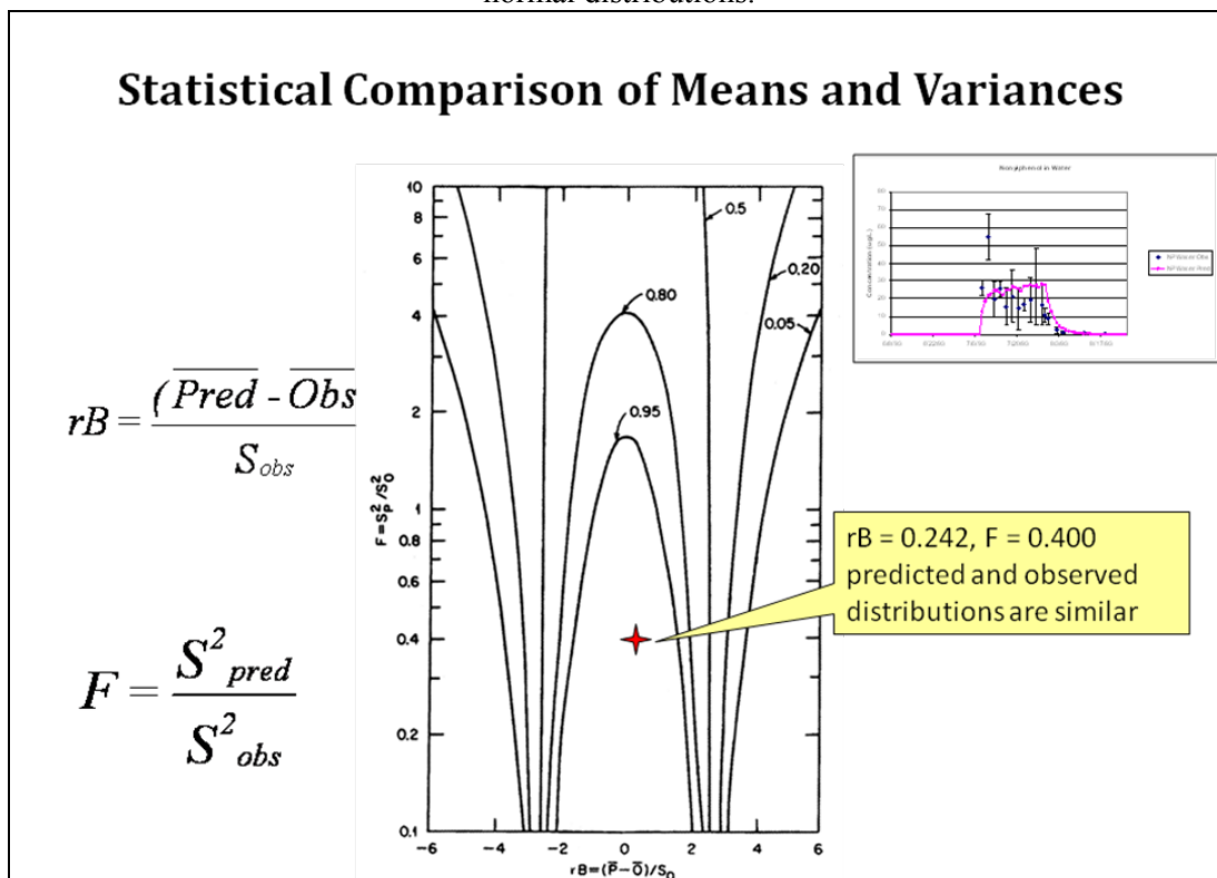
Figure 25. Relative bias and F test to compare means and variances of observed data and predicted results with AQUATOX. The isopleths correspond to the probability that the distributions of predicted and observed, as defined by the combination of the rB and F statistics, are similar. The isopleths assume normal distributions.
