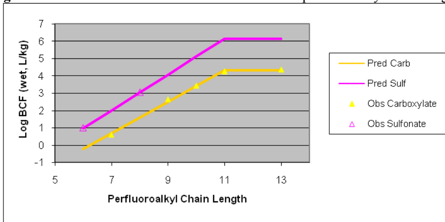
Figure 154. Bioconcentration factors as functions of perfluoroalkyl chain length.
