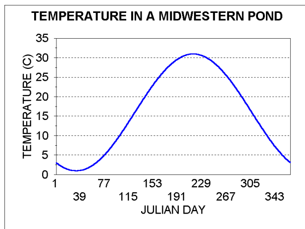
Figure 45. Annual Temperature
