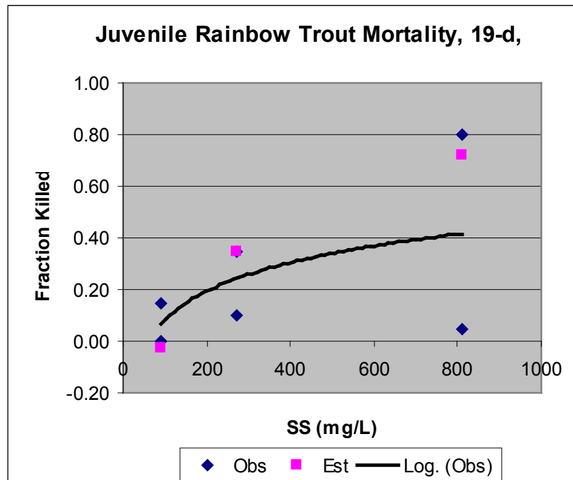
Figure 79. Lethality of suspended sediments to juvenile rainbow trout ( Oncorhynchus mykiss ) using parameters for sensitive species. Data from Berry et al. (2003).
