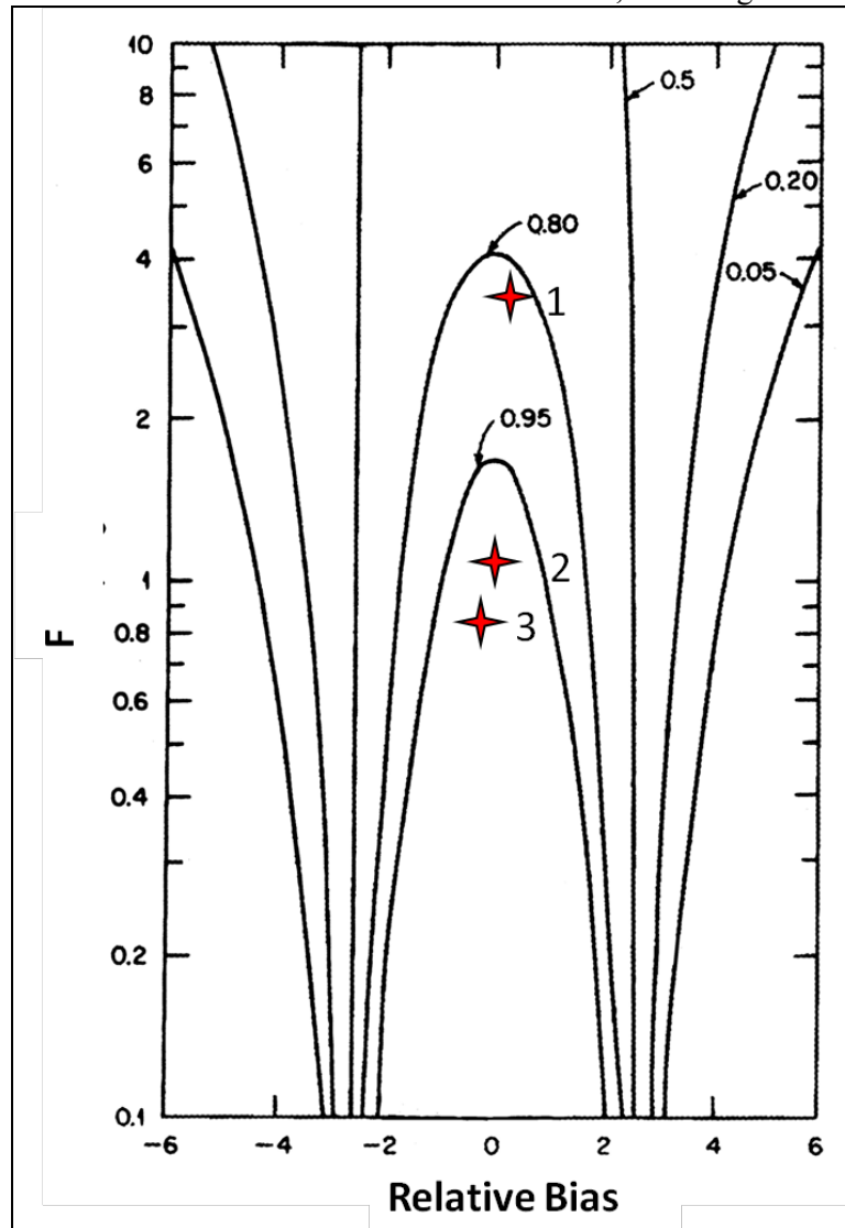
Figure 31. Overlap between model and data distributions based on relative bias and ratio of variances, F ; 1 = Blue Earth River, 2 = Crow Wing River, 3 = Rum River. Isopleths indicate the probability that the predicted and observed distributions are the same, assuming normality.
