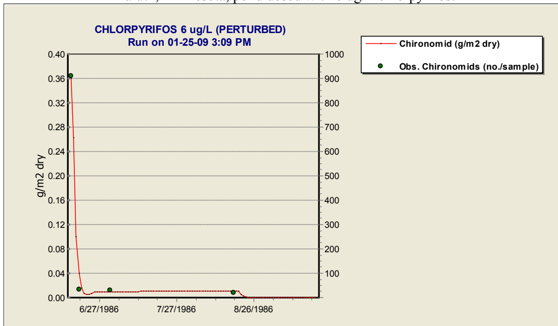
Figure 21. Predicted biomass and observed numbers of chironomid larvae in a Duluth, Minnesota, pond dosed with 6 ug/L chlorpyrifos.
